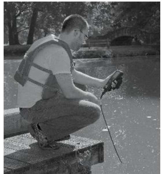
Turbidity can help determine the health of a water body.
